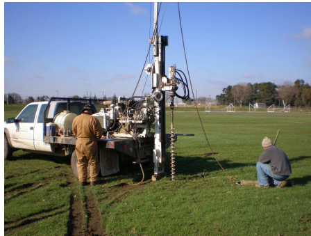
Allied Health Project - Geotechnical Boring Testing at MJC West Campus
