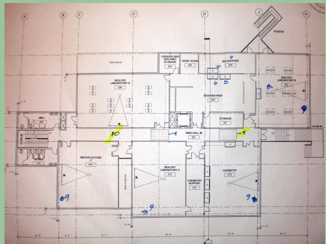
Draft Schematic Design Plan
