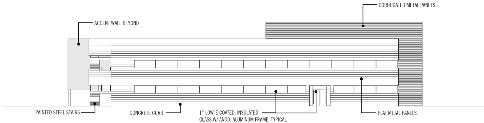
EAST ELEVATION
