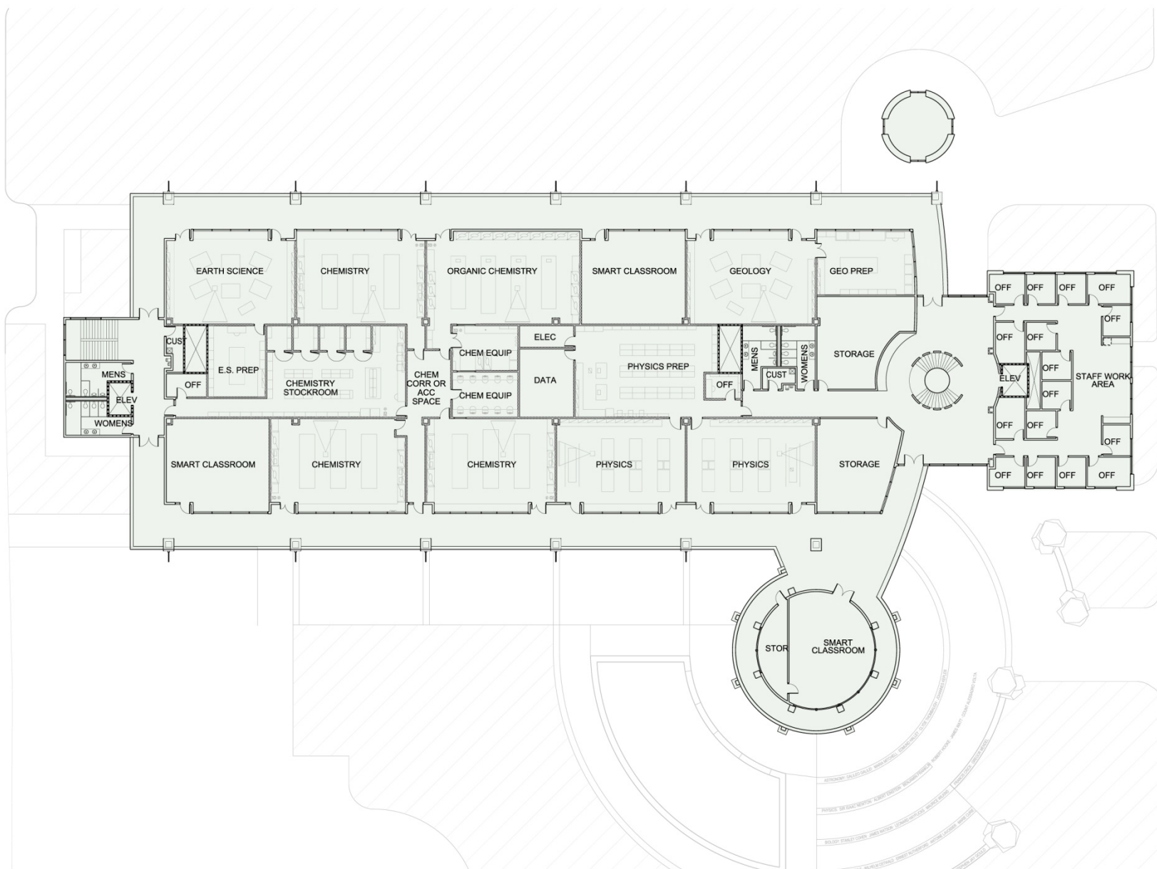
Third Floor Plan – Modesto Junior College Science Community Center
