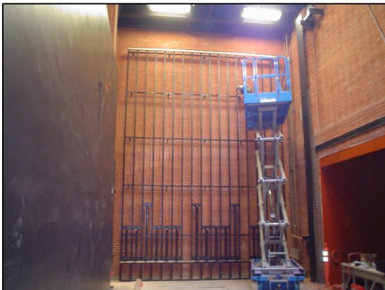
Installing the Little Theater Rigging System
